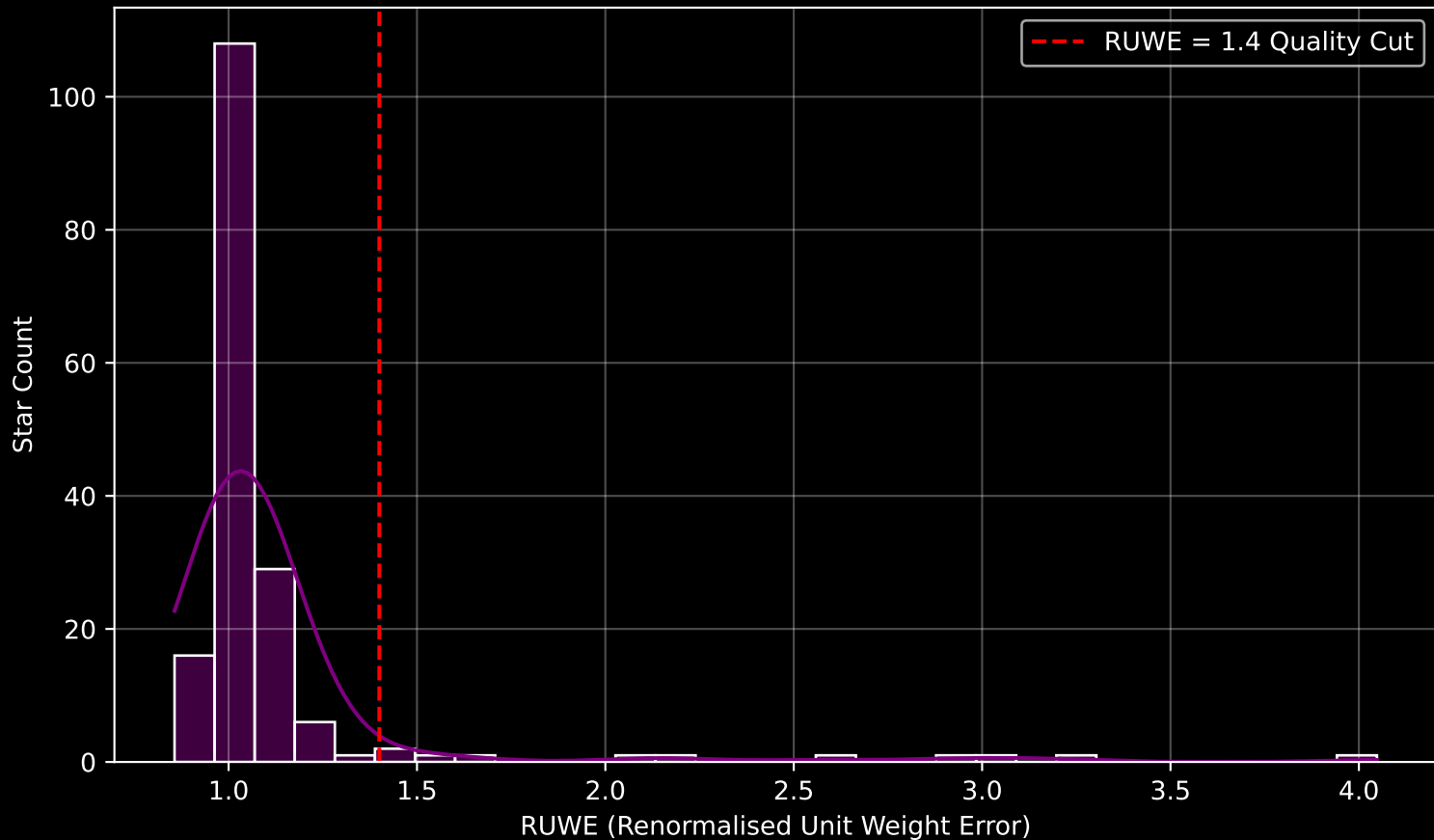
GAPOGEE DR17 Field [109+04] RUWE Distribution (n= 171)
