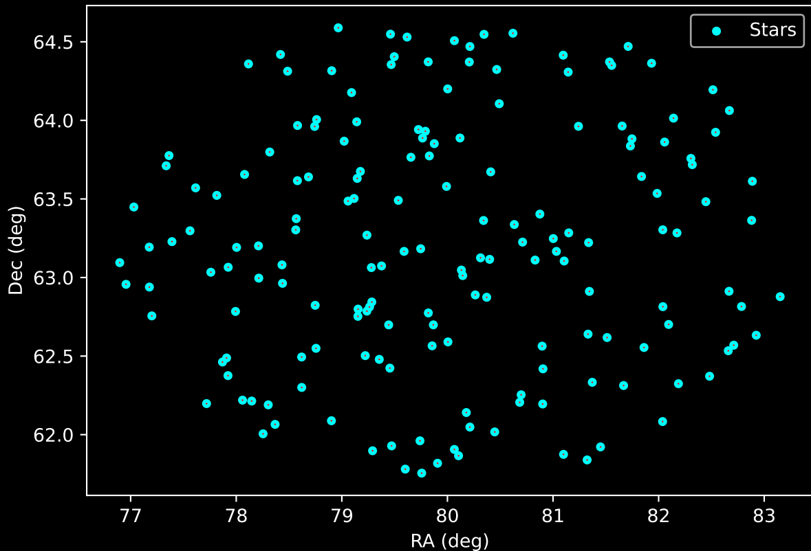
APOGEE DR17 Field: [109+04] Proper Motion Vectors for Gaia Star Field (n= 172)
