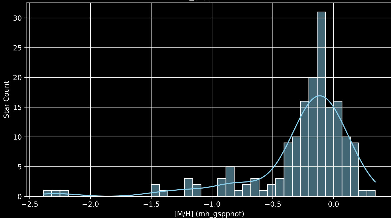
APOGEE DR17 Field: [109+04 [M/H] (mh_gspphot) (n= 169)
