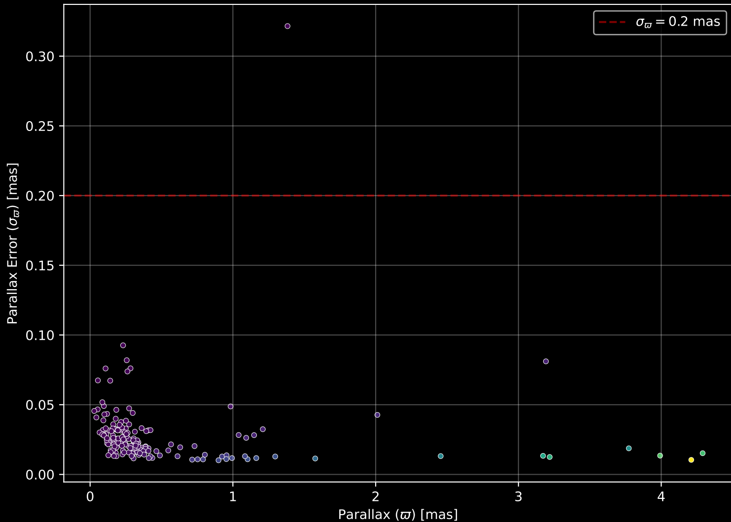
APOGEE DR17 Field: [109+04] Parallax Quality (n= 172)
