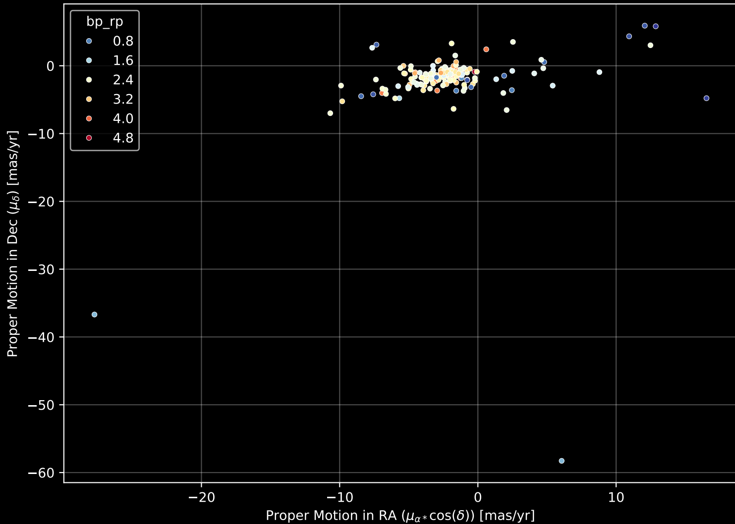
APOGEE DR17 Field: [109+04] Proper Motion Diagram (n= 172)
